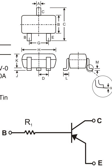
SCHMATIC DIAGRAM
